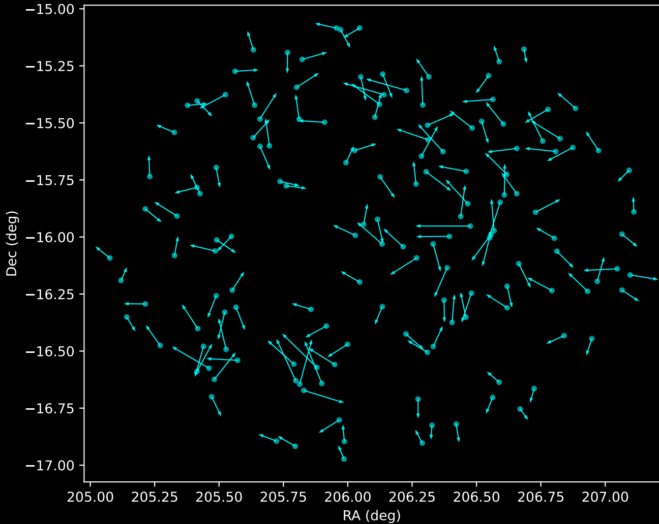
GALAH DR4 Noise Stream Proper Motion Vectors (n=149)
