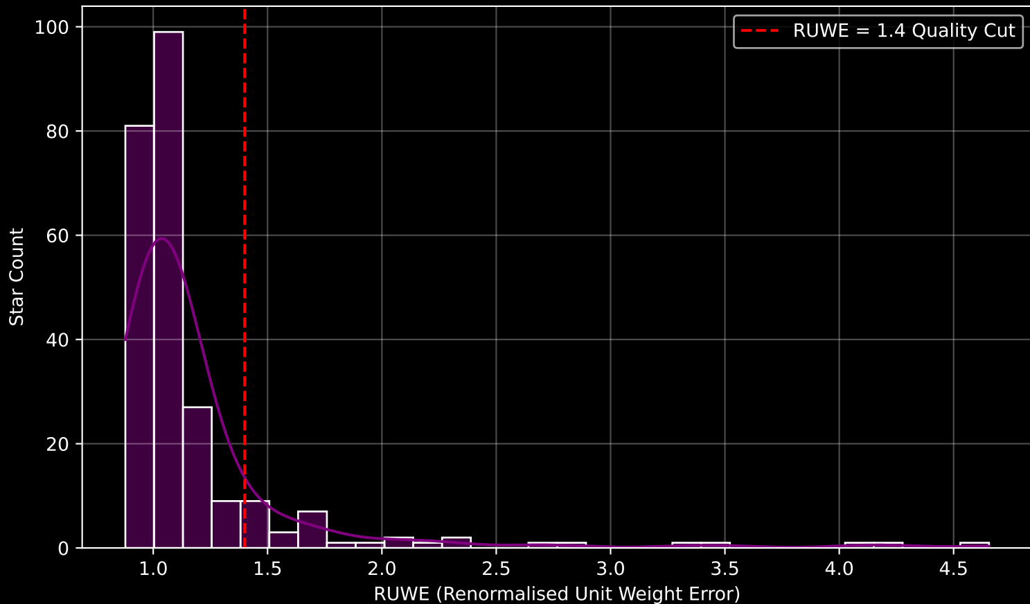
GALAH DR4 Field [8684] RUWE Distribution (n= 249)
