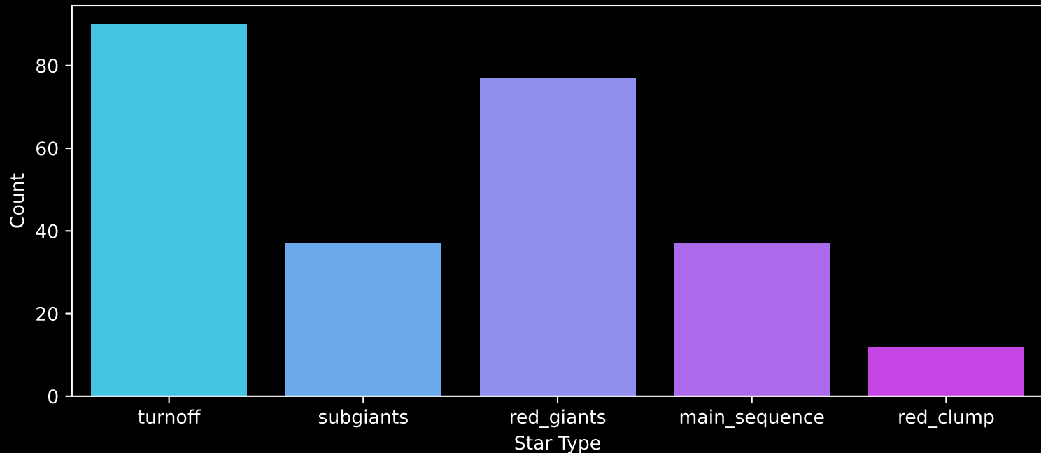
GALAH DR4 Field: [8684] Count plot of Star Type
