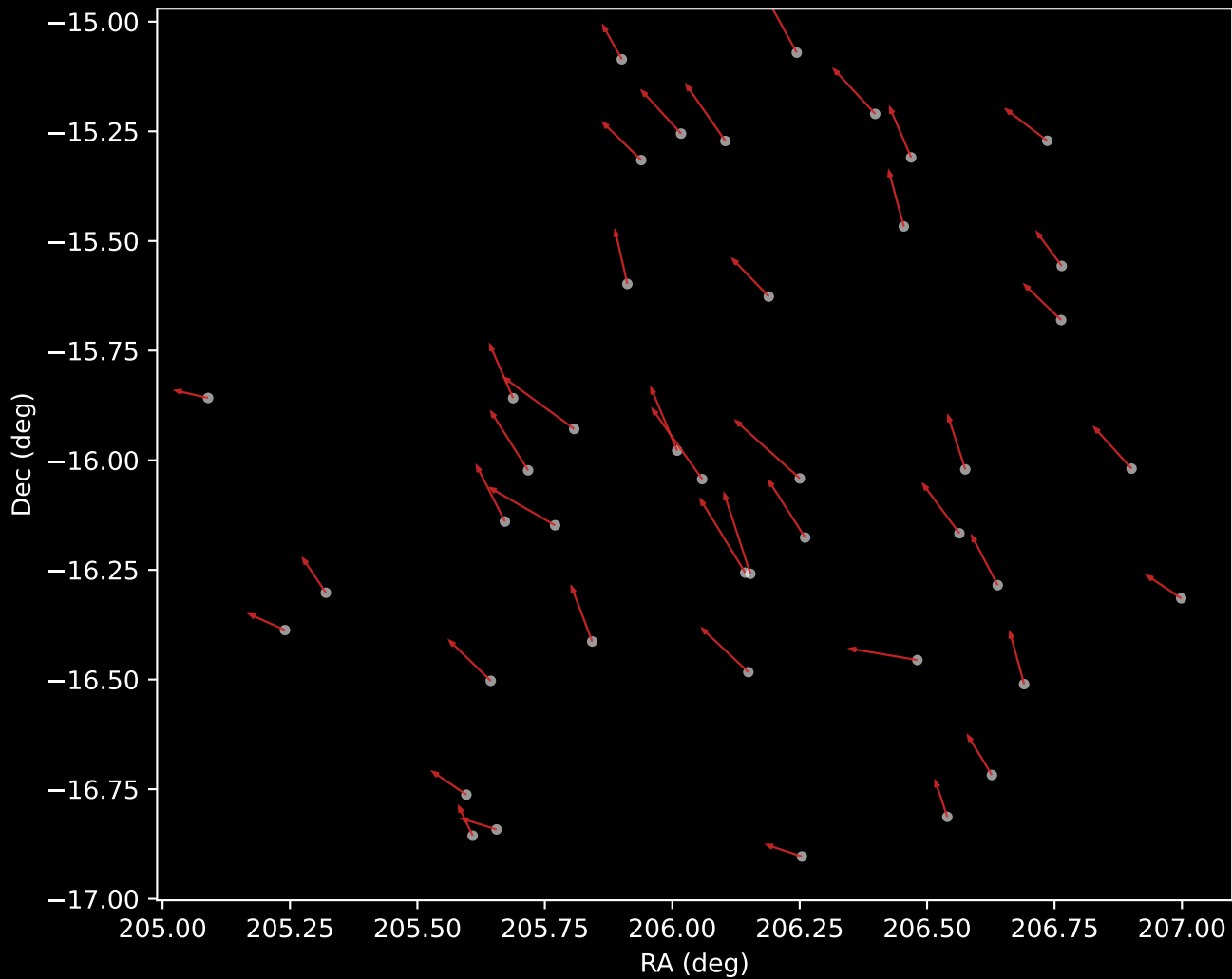
GALAH DR4 Cluster 6 Proper Motion Vectors (n=43)
