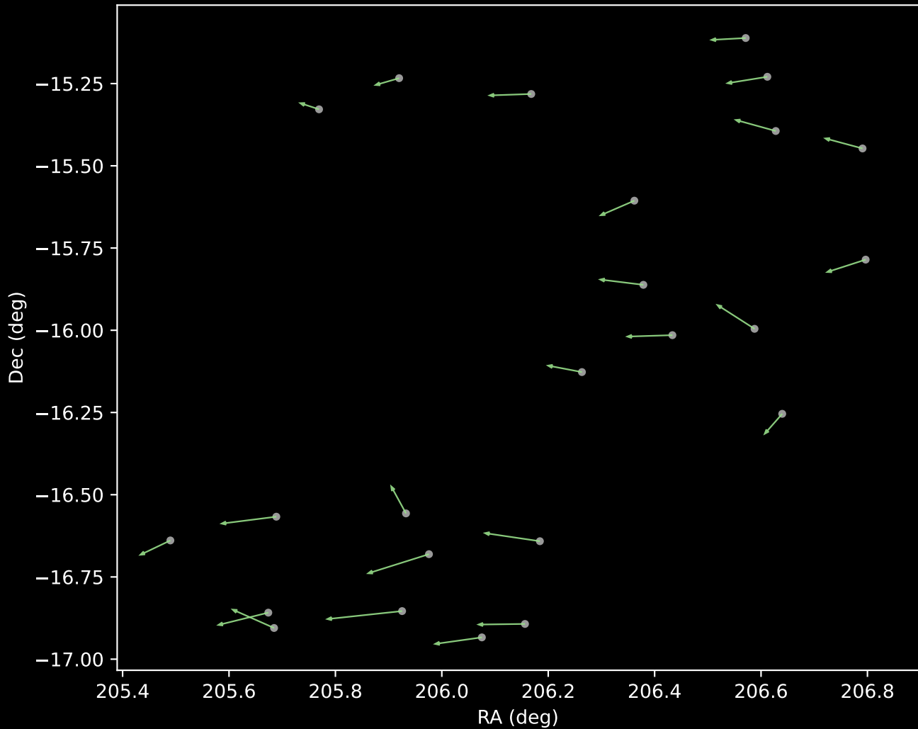
GALAH DR4 Cluster 5 Proper Motion Vectors (n=24)
